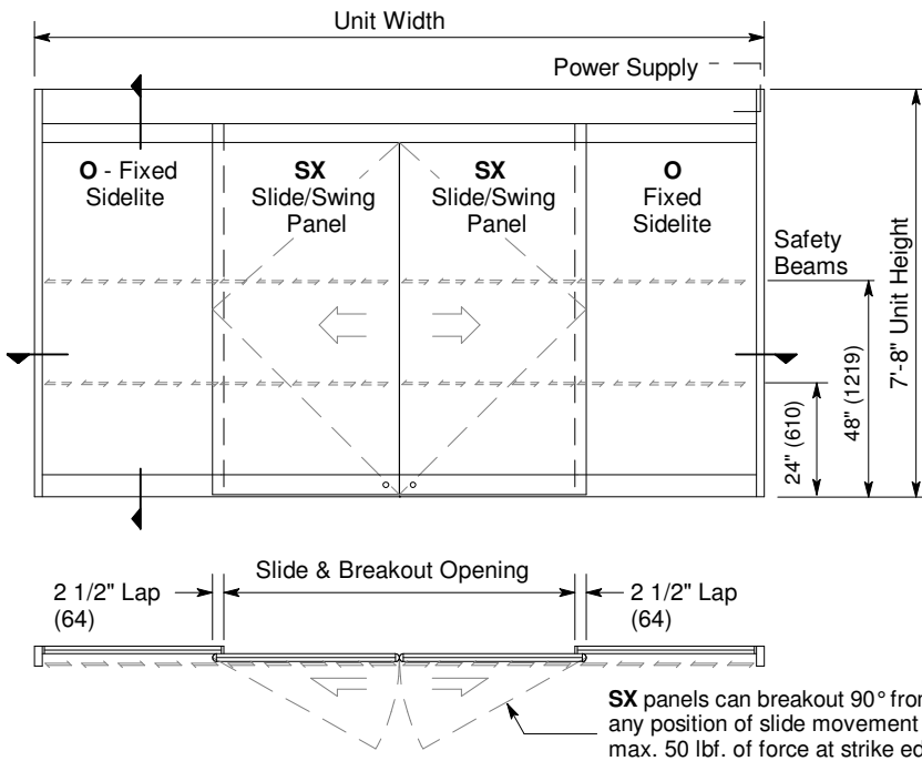
Exterior Elevation and Floor Plan
