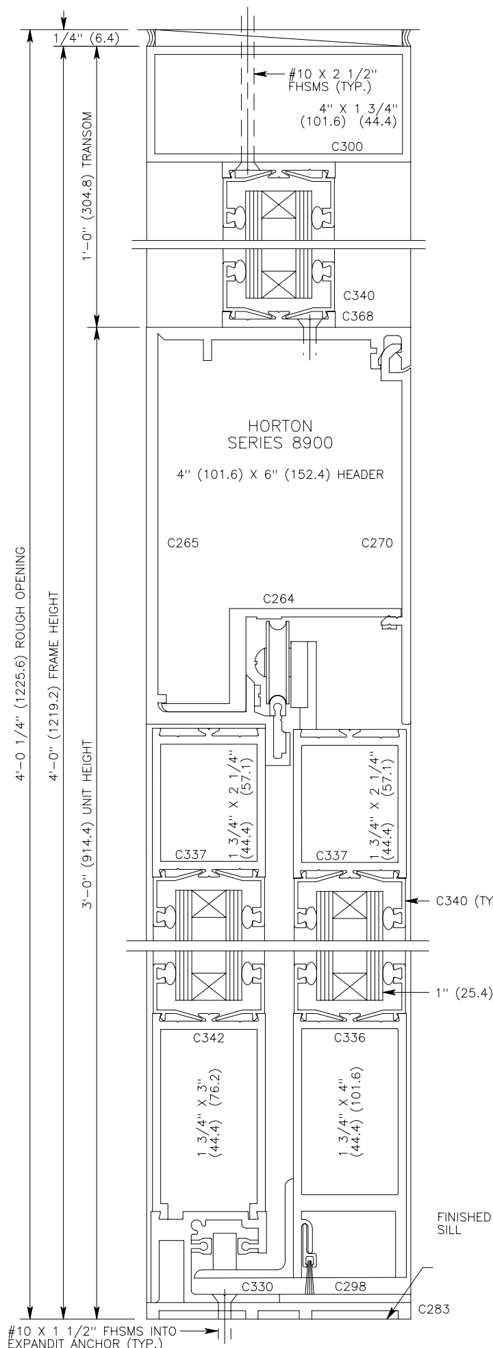
VERTICAL SECTION 1 DOOR SHOWN IN OPEN POSITION
