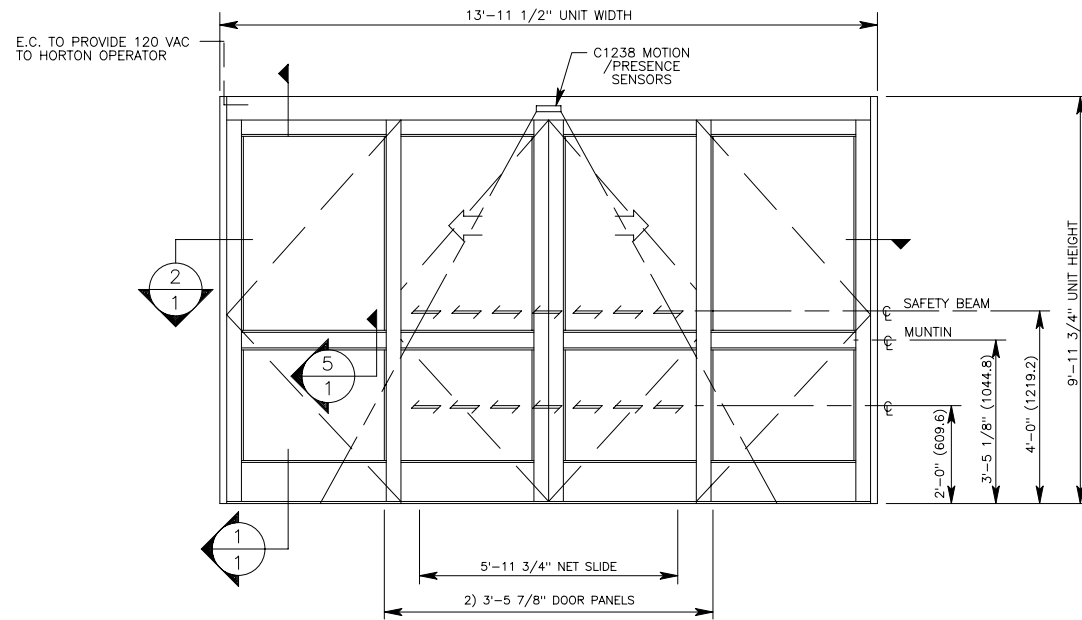
ELEVATION 7 4 THU DR. #23A, 23B, 01C, 01D 1
