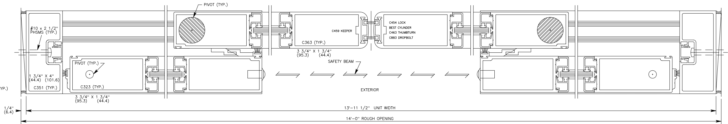
HORIZONTAL SECTION 2 1
