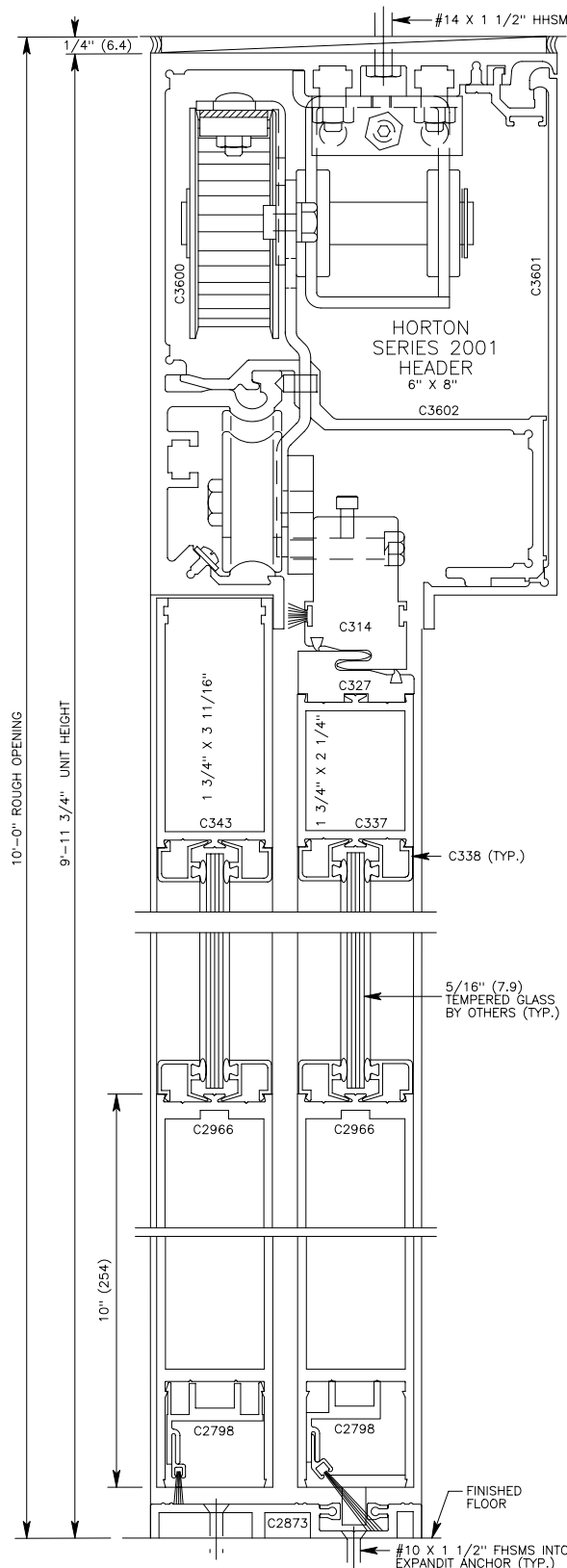
VERTICAL SECTION 1 DOOR SHOWN IN OPEN POSITION 1
