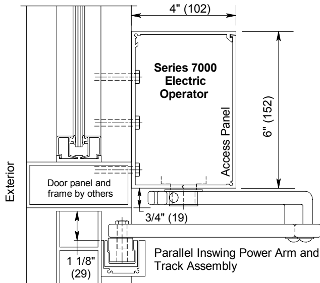
VERTICAL SECTION - CENTER PIVOTED DOOR
