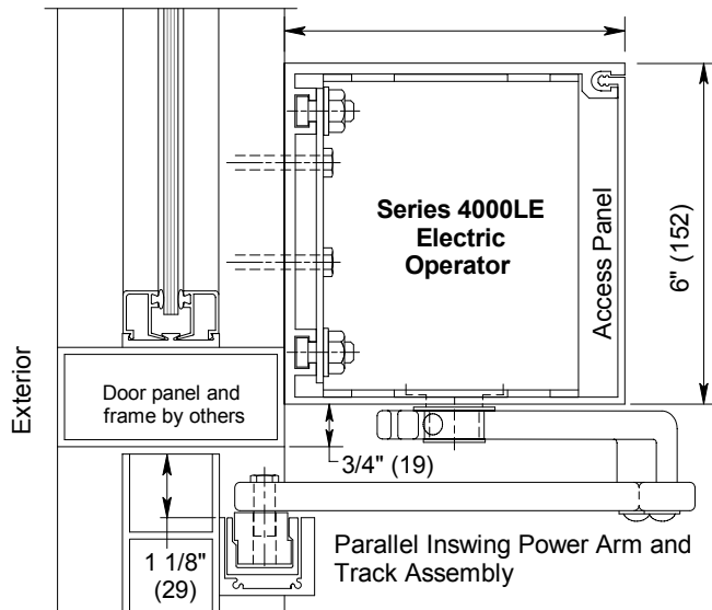
VERTICAL SECTION - CENTER PIVOTED DOOR
