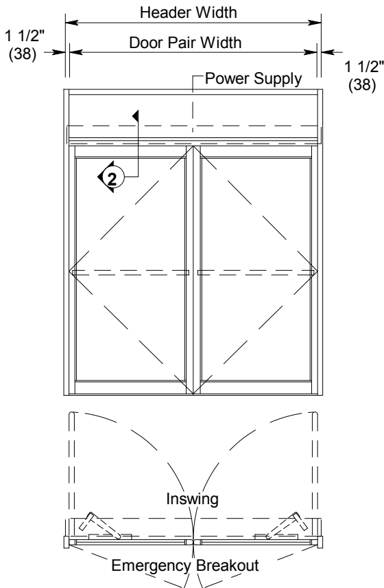
PAIR UNIT - ELEVATION & FLOOR PLAN
