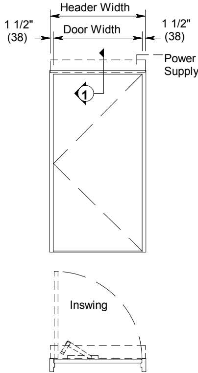
SINGLE UNIT - ELEVATION & FLOOR PLAN
