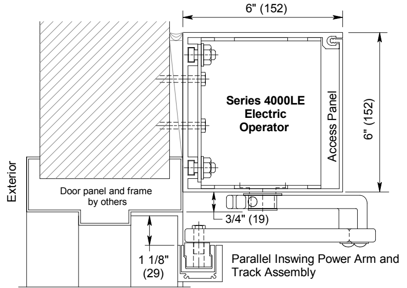
VERTICAL SECTION - BUTT HUNG DOOR
