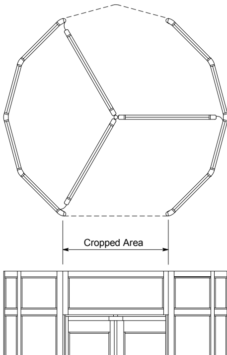
3-Wing Segmented
