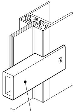
C287-1 Standard Pushbar
