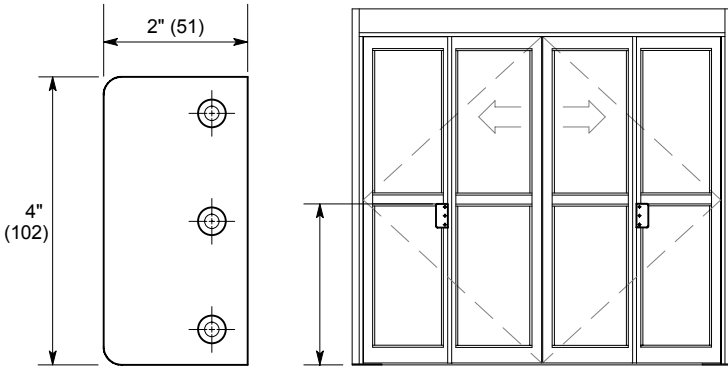
C7641 Pull Handle For manual operation
