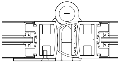
C287-1 Standard Pushbar
