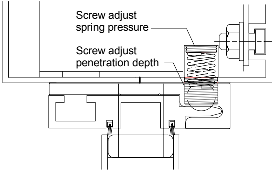
Standard Ball Catch at Header
