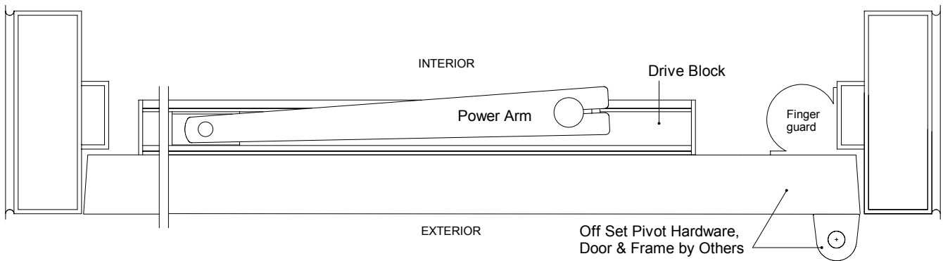
Horizontal Section
