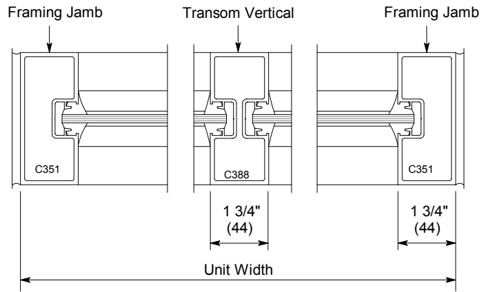
Horizontal Section '3'
