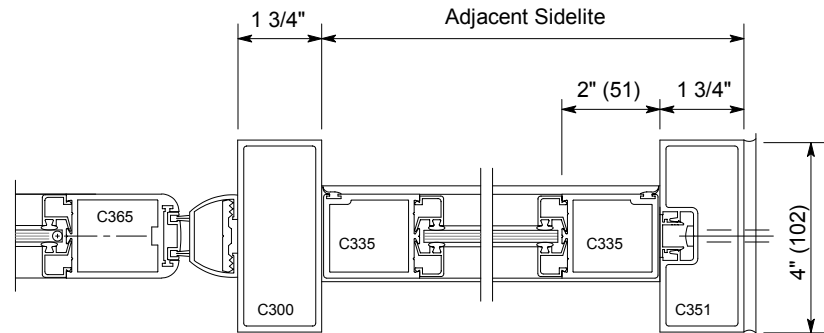
Horizontal Section '1'
