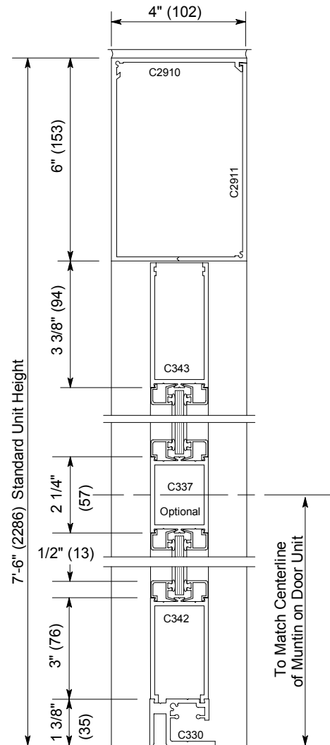
Vertical Section '2'
