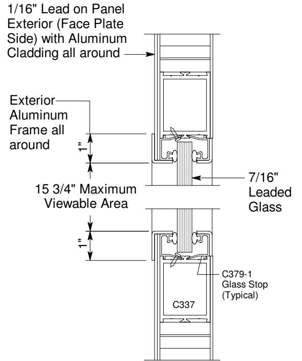
Typical Vertical Section
