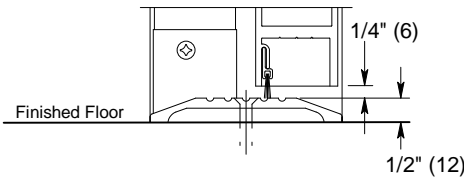
Standard C381 4" (102) Threshold Note: 010 condition shown.
