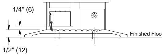
Optional C390 7" (179) Threshold Note: 110 condition shown.
