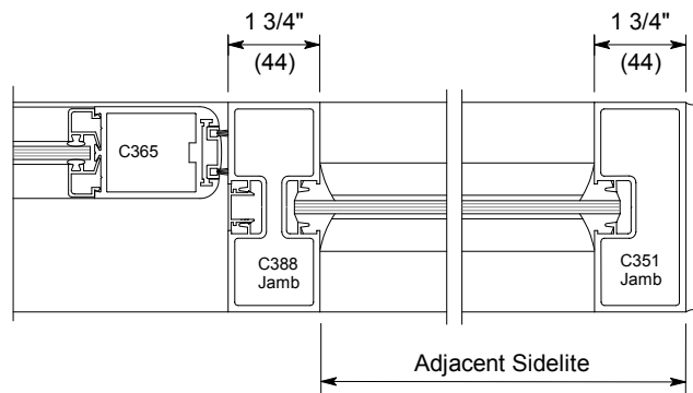
Horizontal Section - '2'
