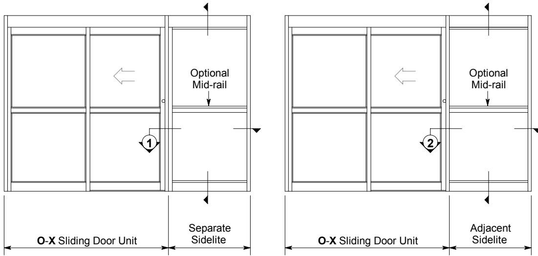
Exterior Elevations
