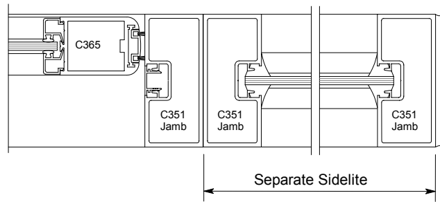
Horizontal Section - '1'
