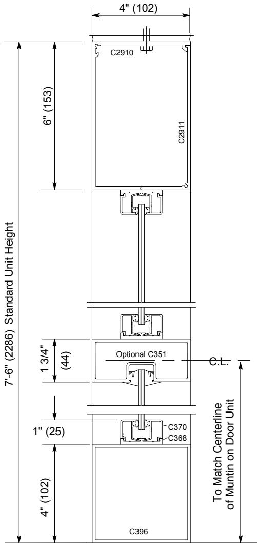
Vertical Section
