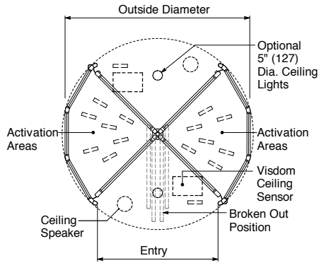
Floor Plan
